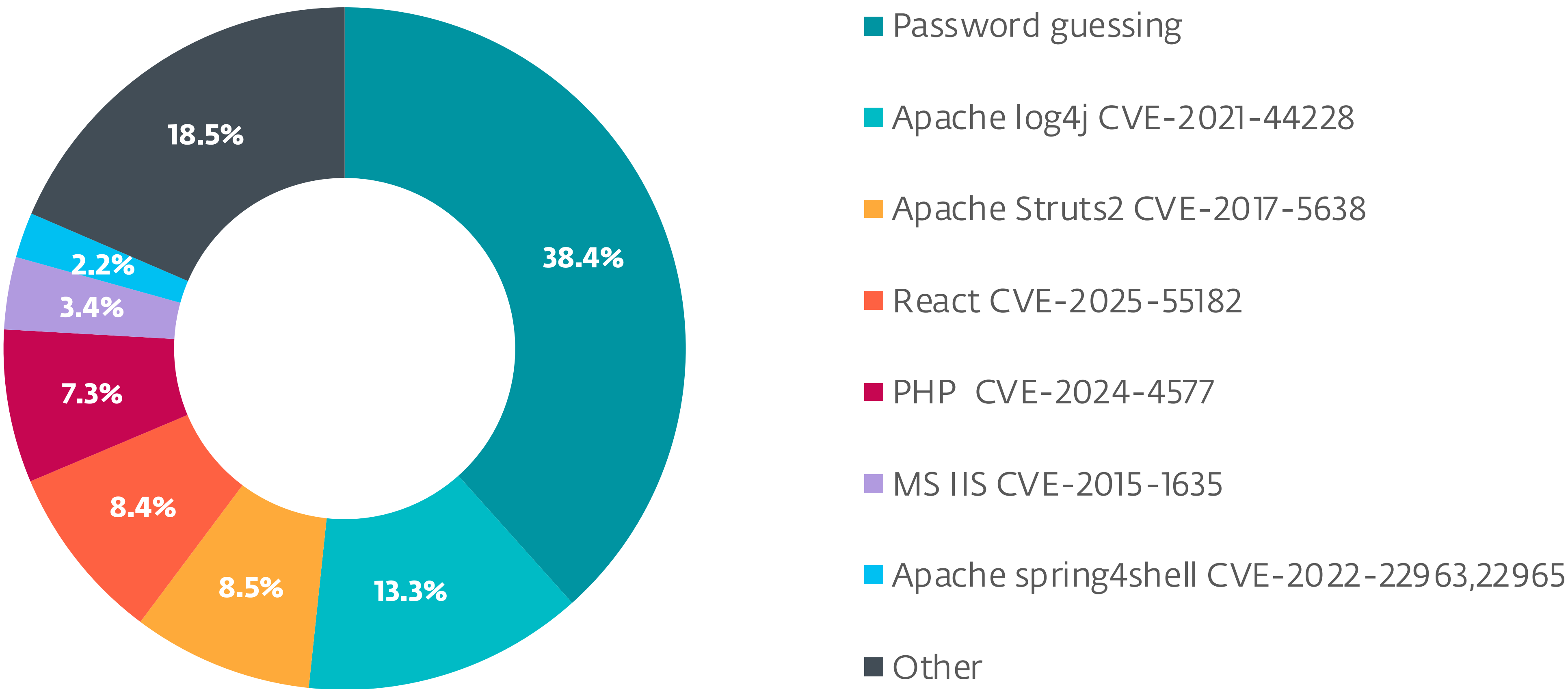
External network intrusion vectors reported by unique clients in H1 2026
