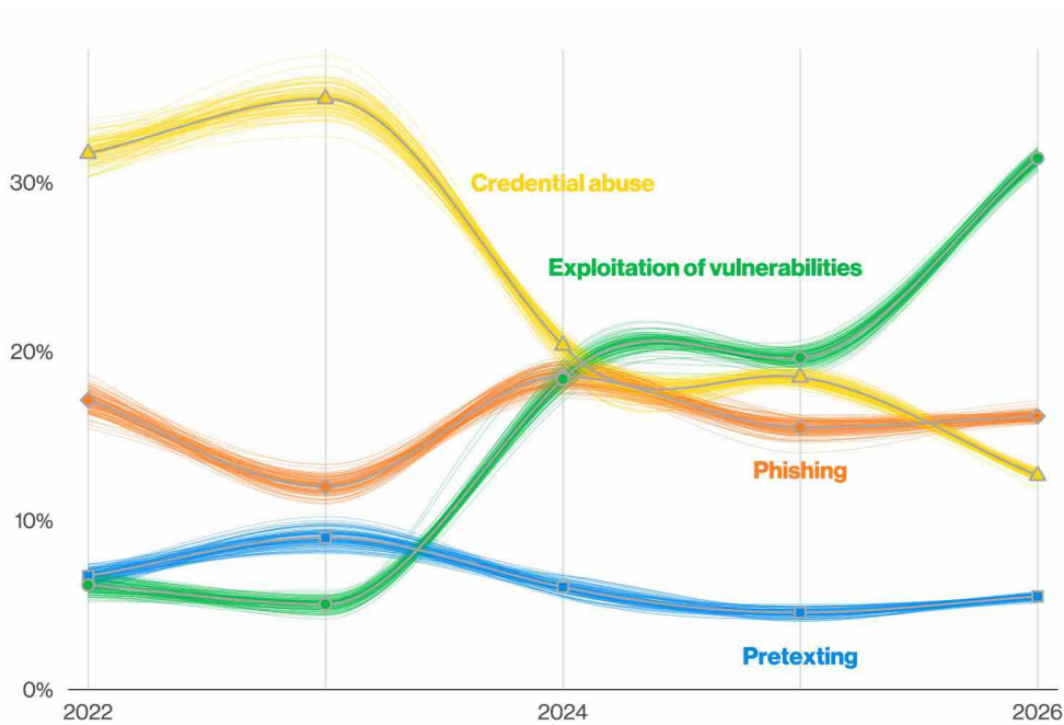
Figure 5. Known initial access vectors in non-Error, non-Misuse breaches over time (n for 2026 dataset=19,905)
