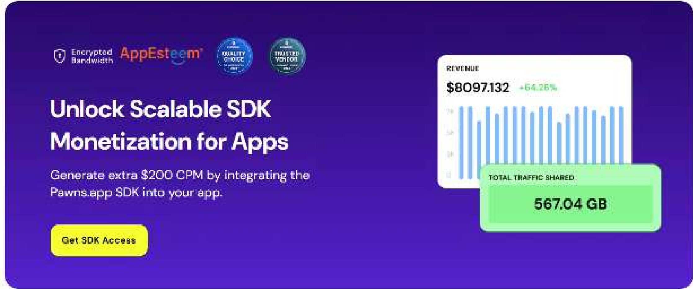
Figure 3 pawns.app.dropper
