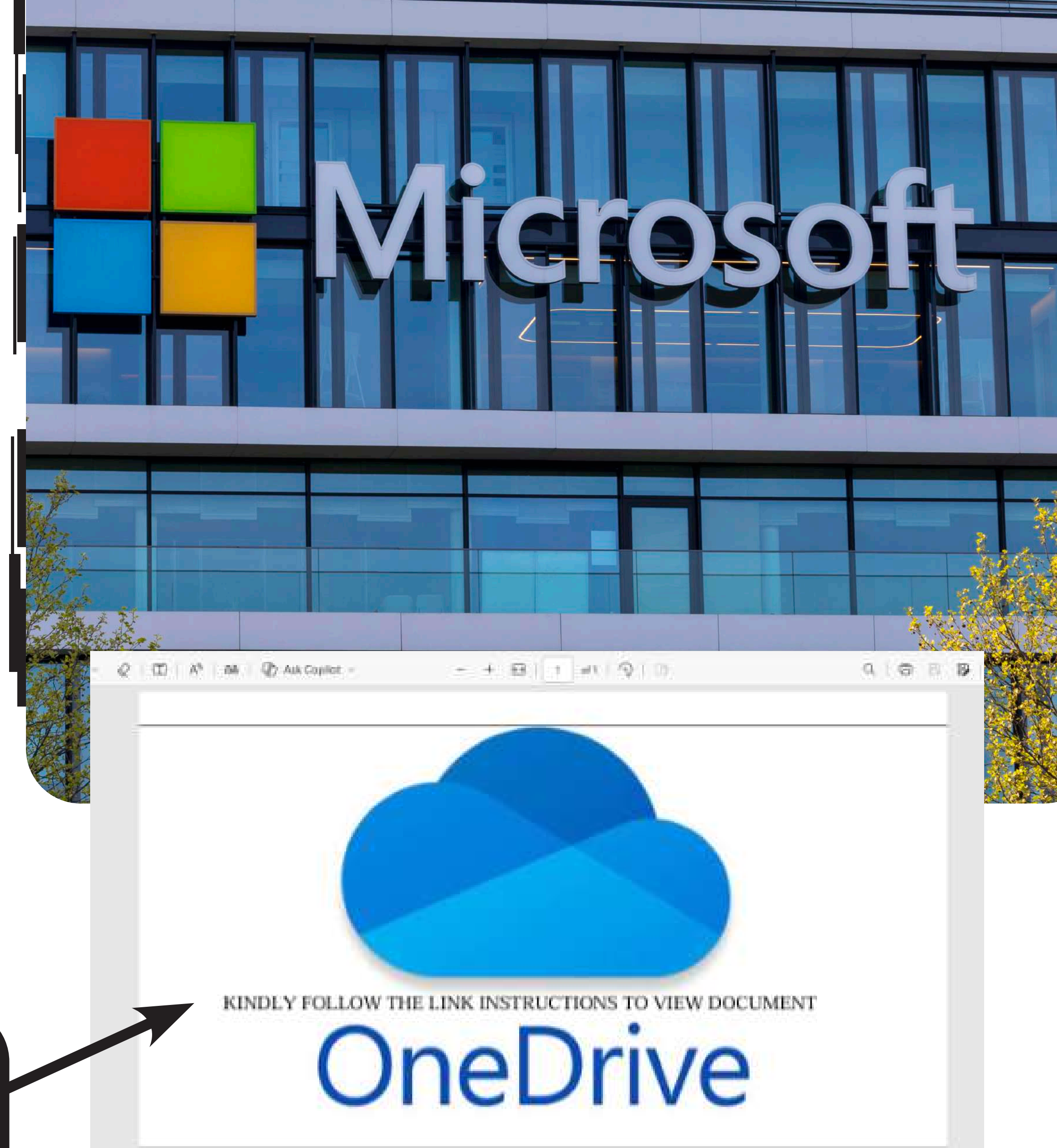
Figure 2 docuphish
